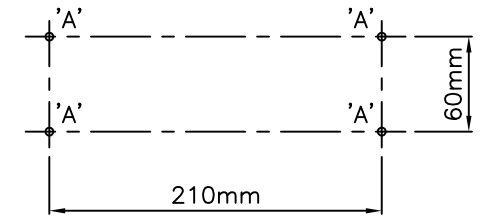
DRILLING DETAIL
